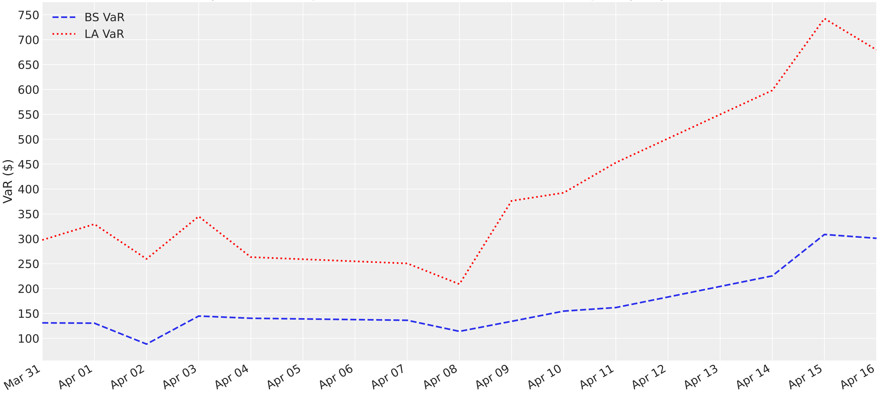
1-Day 99 VaR Comparison between Baseline (BS) and Liquidity Adjusted (LA)
