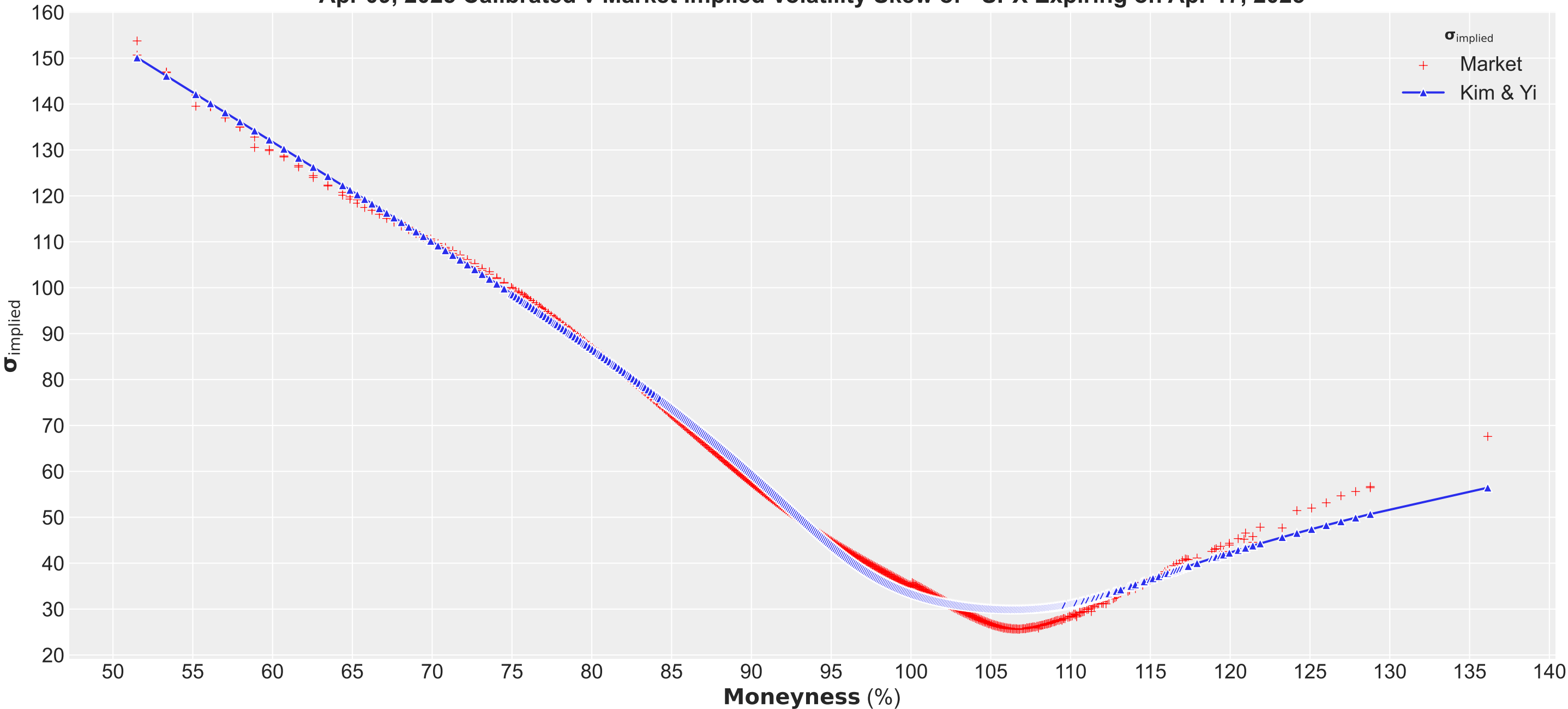
Apr 09, 2025 Calibrated v Market Implied Volatility Skew of ^SPX Expiring on Apr 17, 2025
