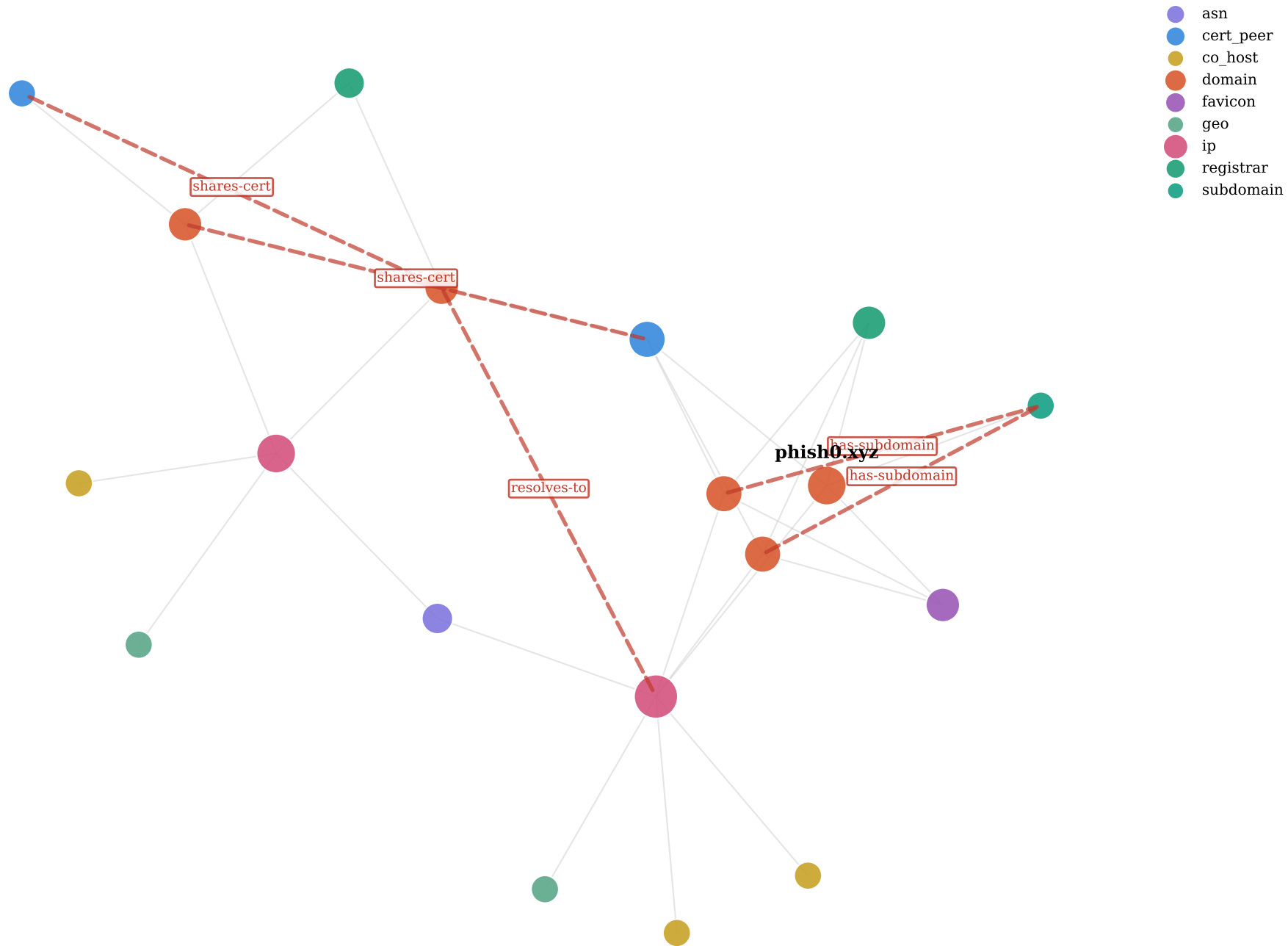
phish0_xyz — predicted missing infrastructure links (dashed red) Top 5 predictions by quantum walk score
