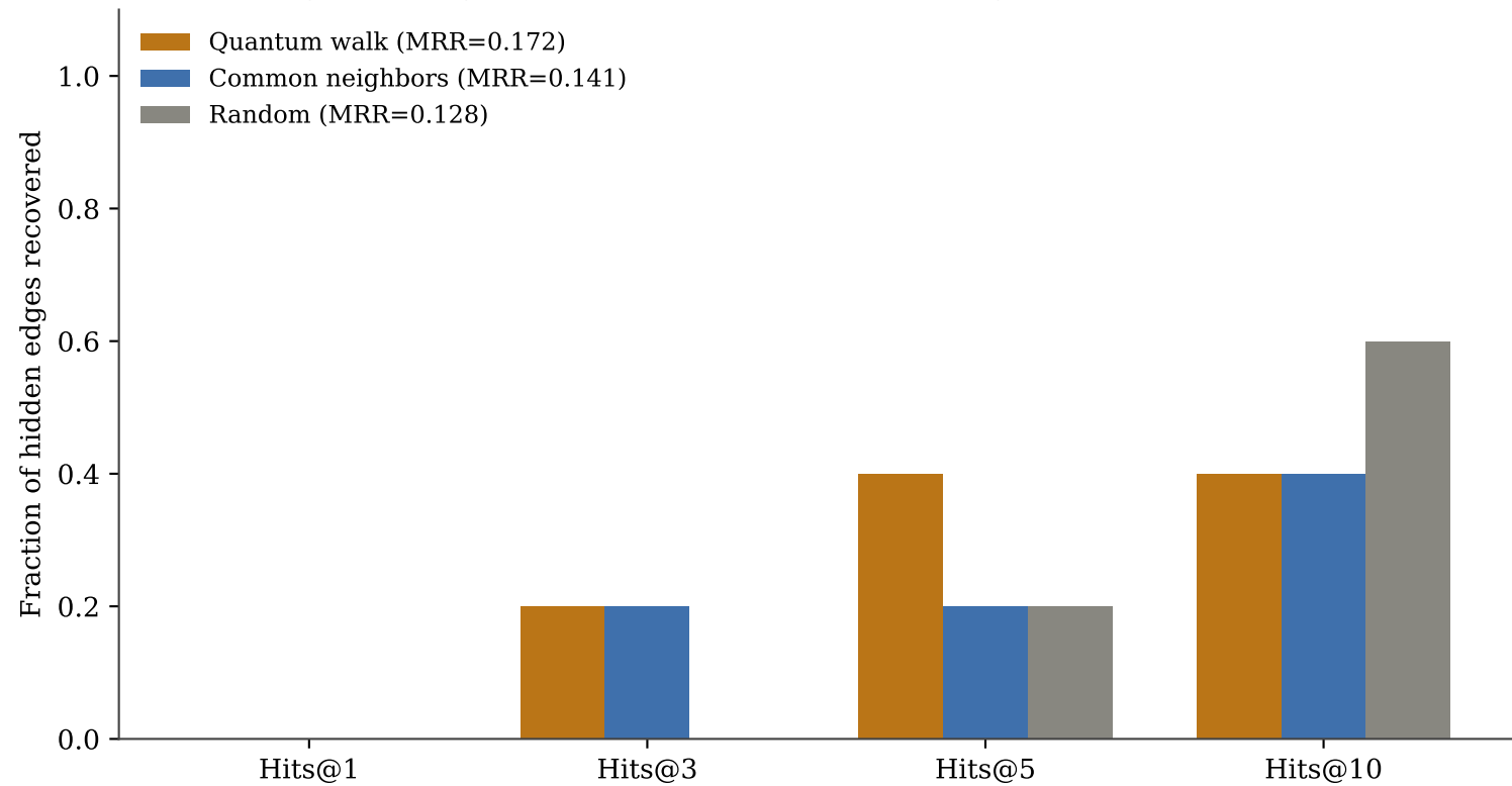
Edge recovery: quantum walk vs baselines (5 edges hidden from 26 total)
