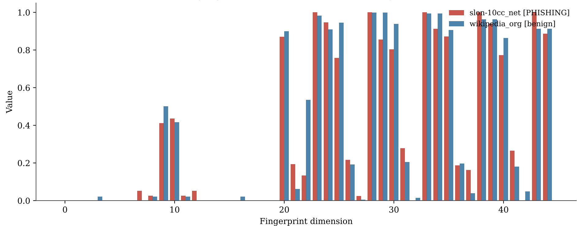
\phi(G) fingerprint comparison — cosine distance = 0.0111 Larger gaps between bars = more structurally distinct
