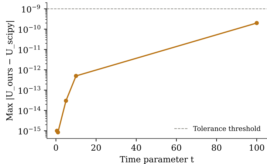
(a) Cross-validation vs scipy.expm
