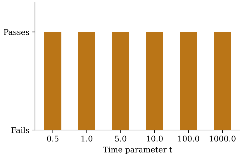
(b) Unitarity check ( U \cdot U^\dagger = I )
