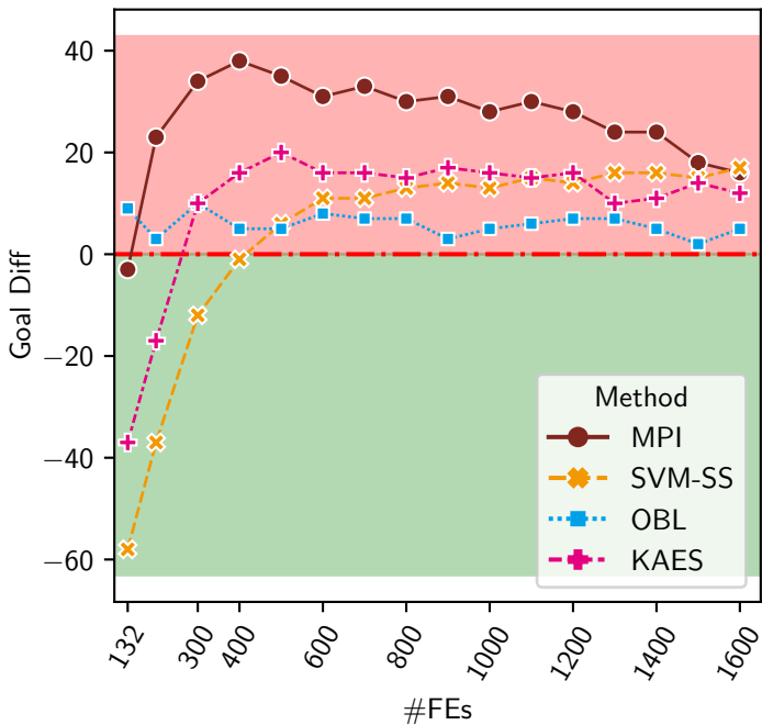
Goal Diff on BRKGA
