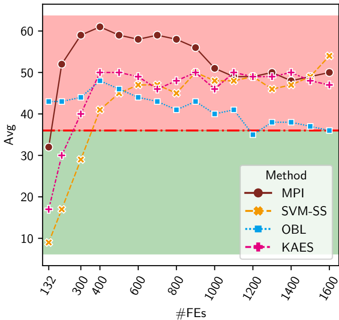
Avg on BRKGA
