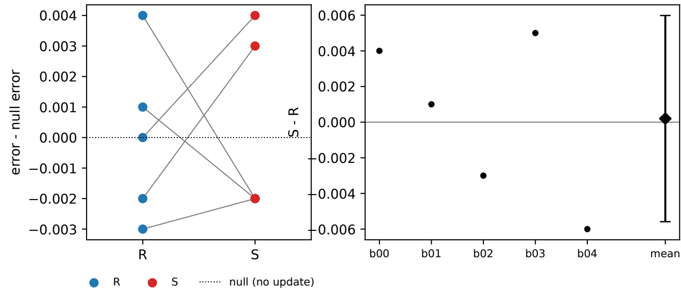
graph_unaudited: eval_ood error change against null (5 blocks)
