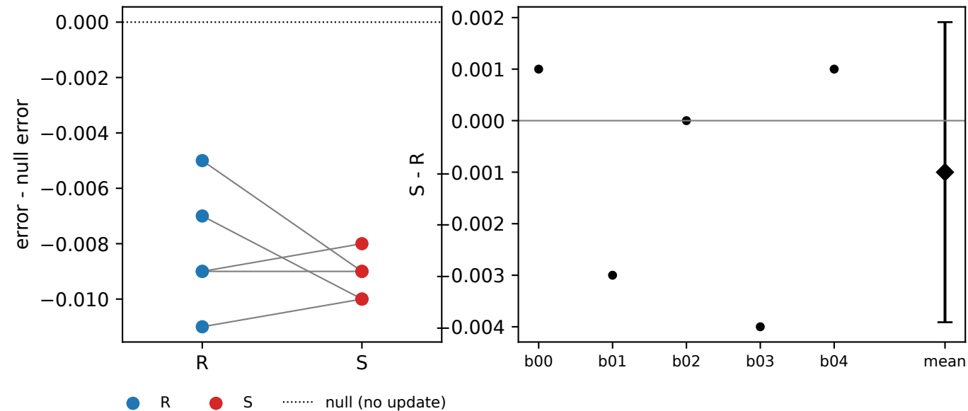
graph_unaudited_llama3.2-3b: eval_ood error change against null (5 blocks)
