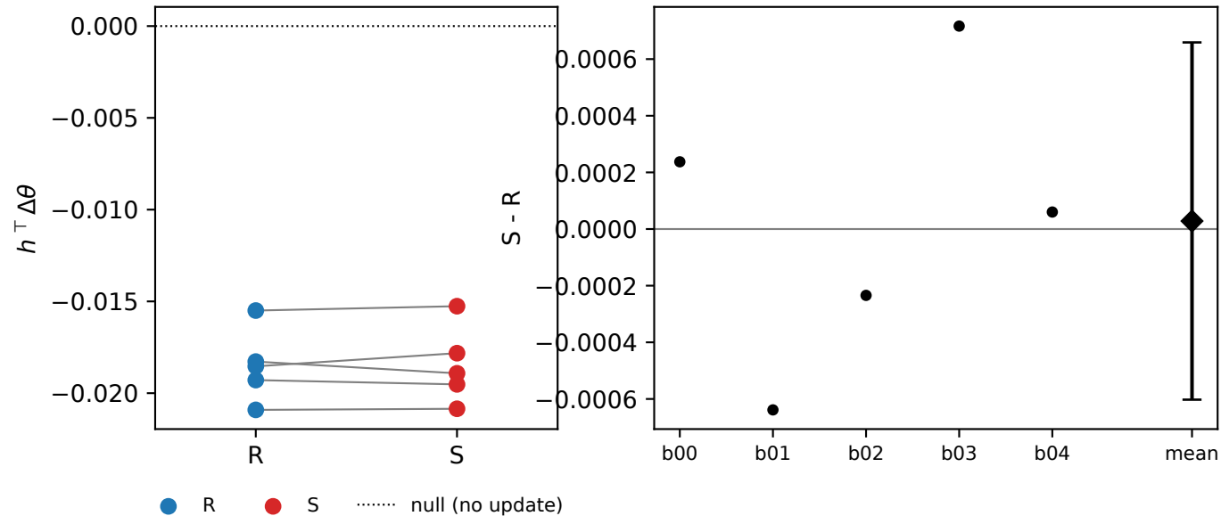
graph_unaudited_llama3.2-3b: projection of the one-step update on h (5 blocks)
