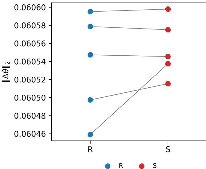
graph_unaudited_qwen3-4b: one-step displacement (5 blocks)
