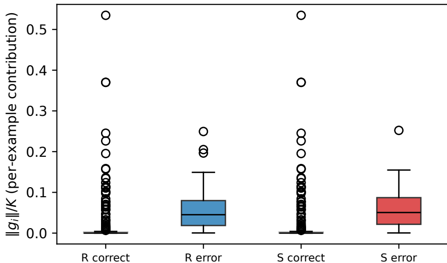
graph_unaudited_qwen3-4b: per-example gradient contributions, all blocks
