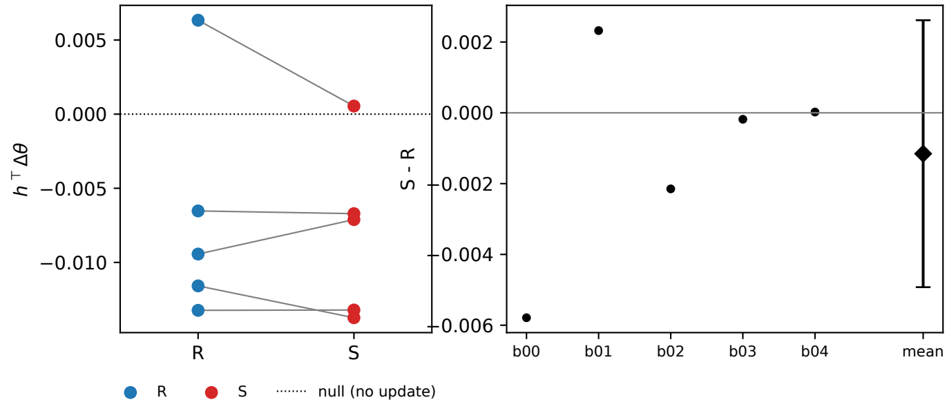
graph_unaudited_qwen3-4b: projection of the one-step update on h (5 blocks)
