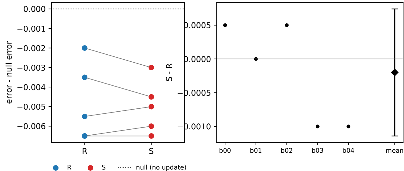
Qwen3-1.7B one-step: ID error change against null
