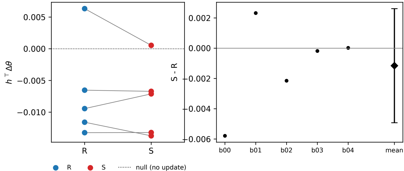
Qwen3-4B one-step: projection on h
