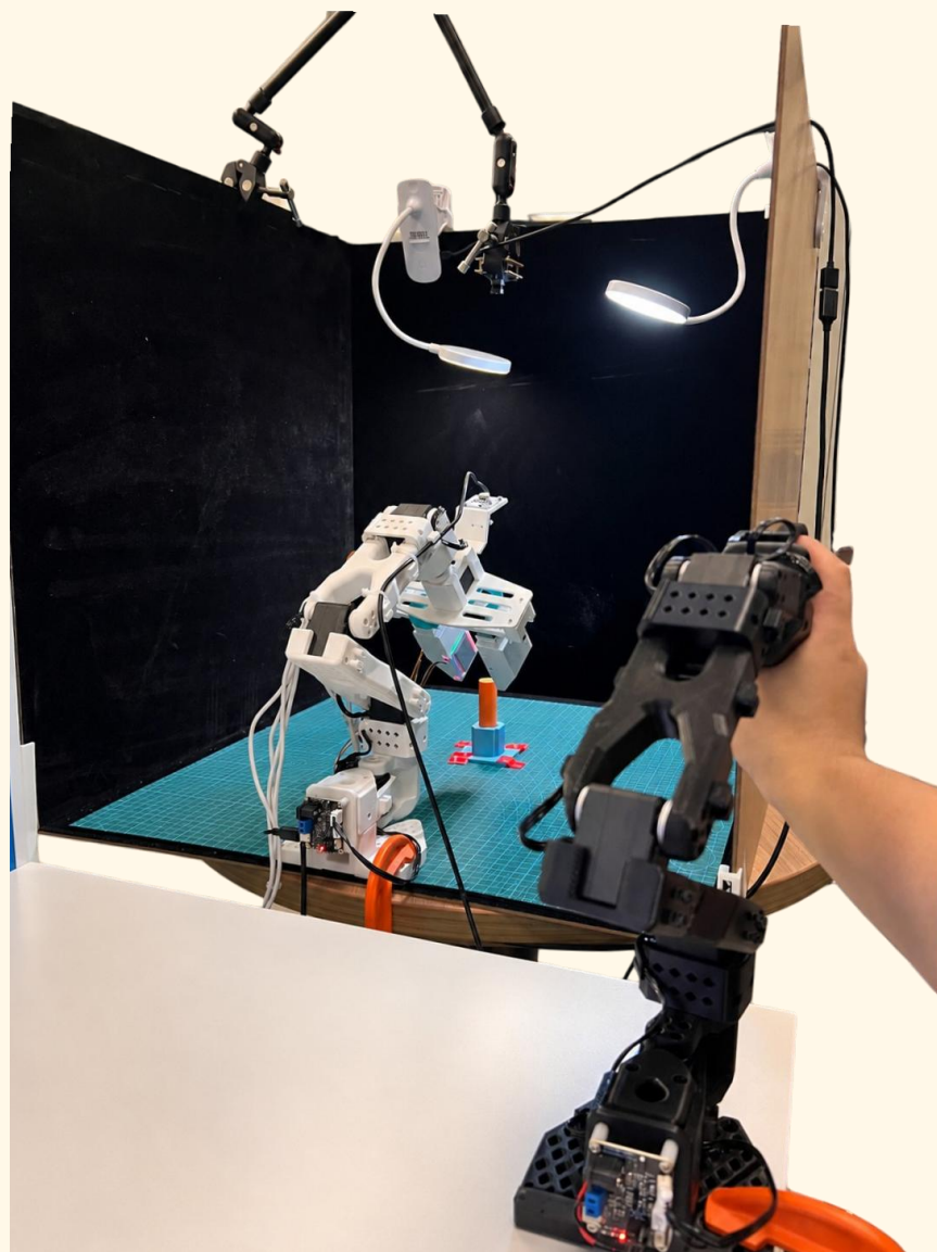
Leader-follower teleoperation
