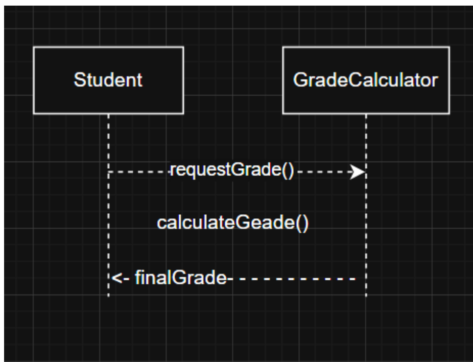
Sequence Diagram:
