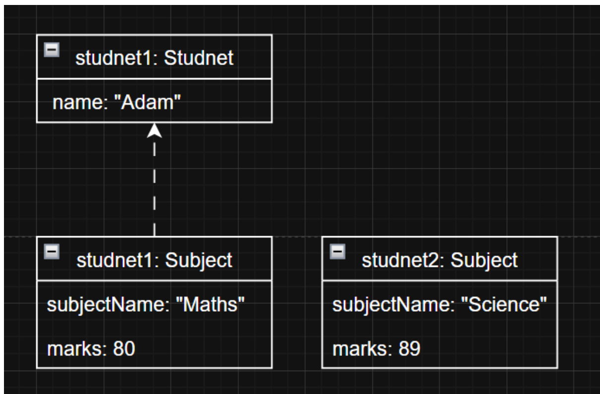
Object Diagram:
