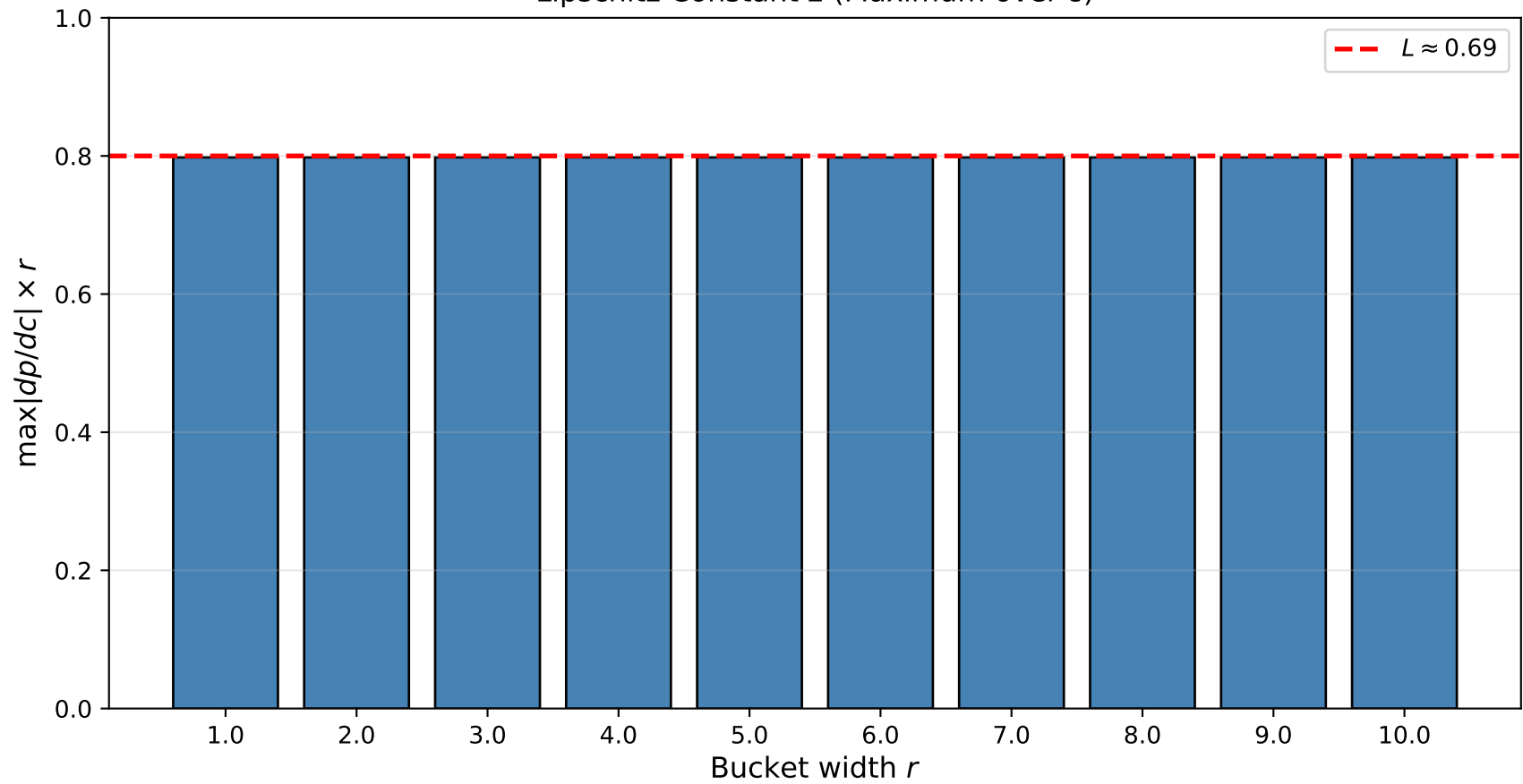
Lipschitz Constant L (Maximum over c )
