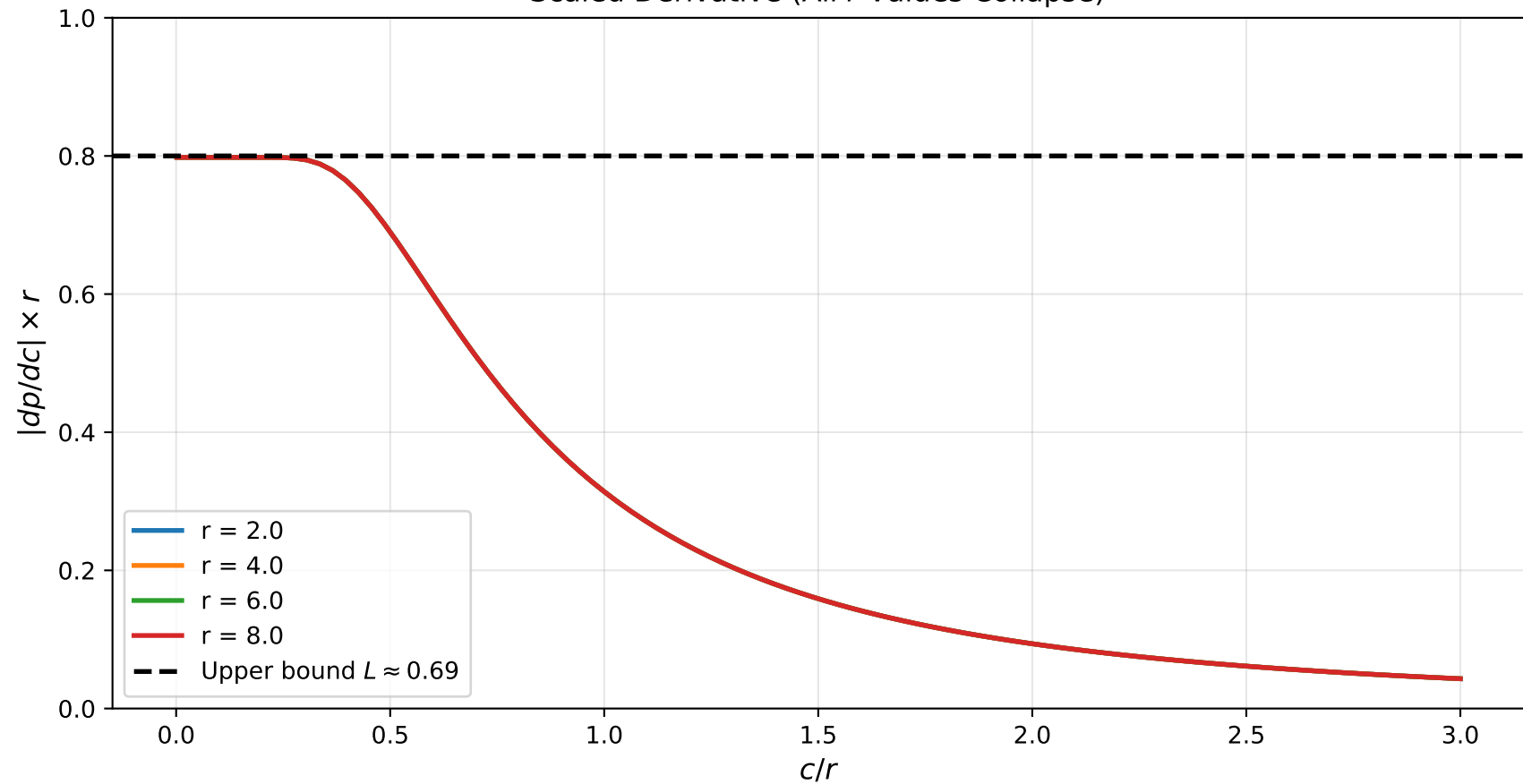
Scaled Derivative (All r Values Collapse)
