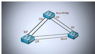
Рис. 1: Spanning Tree Protocol
