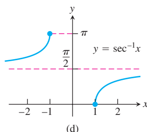
FIGURE 1.66 Graphs of the six basic inverse trigonometric functions.
