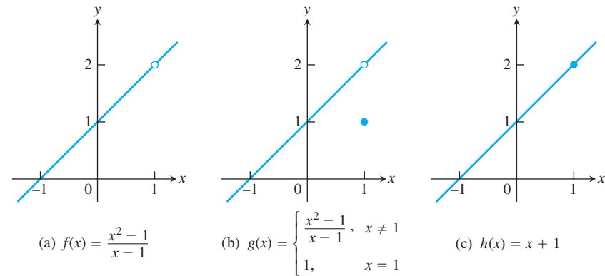
FIGURE 2.8 The limits of f(x) , g(x) , and h(x) all equal 2 as x approaches 1. However, only h(x) has the same function value as its limit at x = 1 (Example 2).
