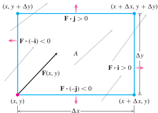
FIGURE 16.26 The rate at which the fluid leaves the rectangular region A across the bottom edge in the direction of the outward normal -\mathbf{j} is approximately \mathbf{F}(x, y) \cdot (-\mathbf{j}) \Delta x , which is negative for the vector field \mathbf{F} shown here. To approximate the flow rate at the point (x, y) , we calculate the (approximate) flow rates across each edge in the directions of the red arrows, sum these rates, and then divide the sum by the area of A . Taking the limit as \Delta x \rightarrow 0 and \Delta y \rightarrow 0 gives the flow rate per unit area.
