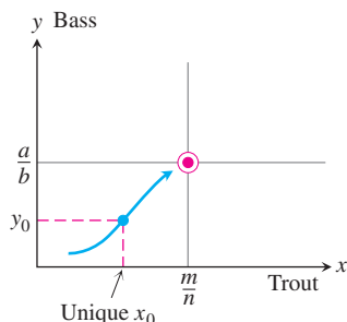
FIGURE 9.36 For any y < a/b only one solution trajectory leads to the rest point (m/n, a/b) .
