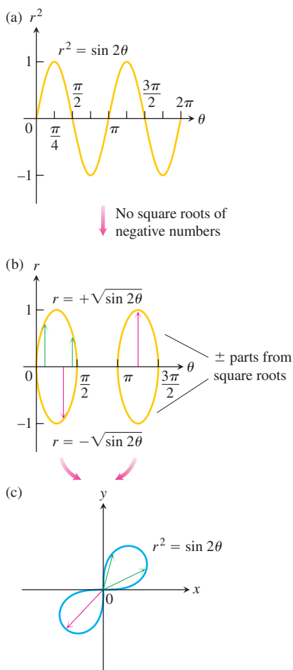
FIGURE 11.29 To plot r = f(\theta) in the Cartesian r\theta -plane in (b), we first plot r^2 = \sin 2\theta in the r^2\theta -plane in (a) and then ignore the values of \theta for which \sin 2\theta is negative. The radii from the sketch in (b) cover the polar graph of the lemniscate in (c) twice (Example 3).
