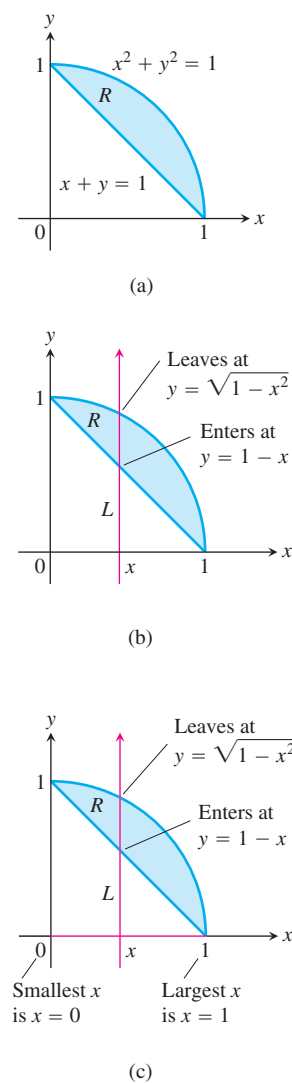
FIGURE 15.14 Finding the limits of integration when integrating first with respect to y and then with respect to x .
