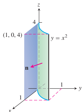
FIGURE 16.51 Finding the flux through the surface of a parabolic cylinder (Example 4).
