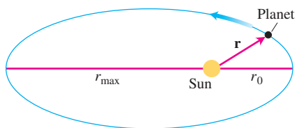
FIGURE 13.36 The length of the major axis of the ellipse is 2a = r_0 + r_{\max} .
