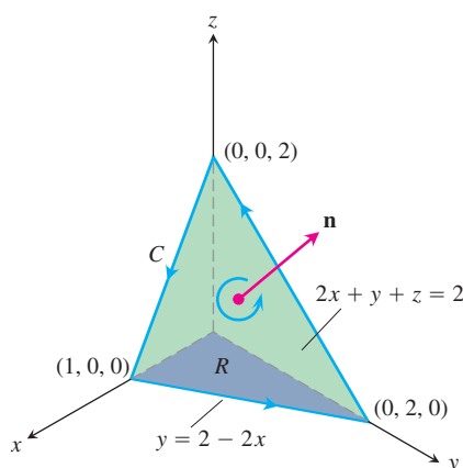
FIGURE 16.62 The planar surface in Example 7.
