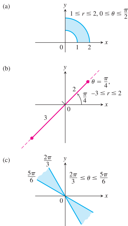
FIGURE 11.23 The graphs of typical inequalities in r and \theta (Example 3).
