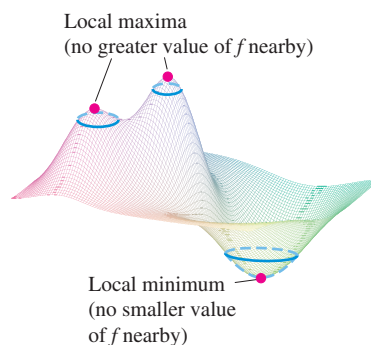
FIGURE 14.40 A local maximum occurs at a mountain peak and a local minimum occurs at a valley low point.
