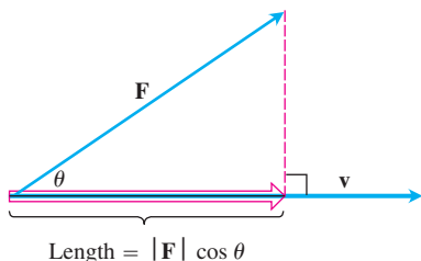
FIGURE 12.19 The magnitude of the force \mathbf{F} in the direction of vector \mathbf{v} is the length |\mathbf{F}| \cos \theta of the projection of \mathbf{F} onto \mathbf{v} .
