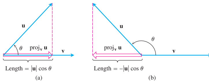
FIGURE 12.25 The length of \text{proj}_{\mathbf{v}} \mathbf{u} is (a) |\mathbf{u}| \cos \theta if \cos \theta \geq 0 and (b) -|\mathbf{u}| \cos \theta if \cos \theta < 0 .
