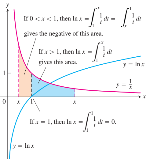
FIGURE 7.1 The graph of y = \ln x and its relation to the function y = 1/x, x > 0 . The graph of the logarithm rises above the x -axis as x moves from 1 to the right, and it falls below the axis as x moves from 1 to the left.
