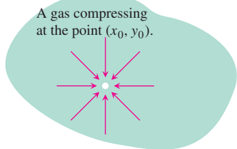
FIGURE 16.27 If a gas is expanding at a point (x_0, y_0) , the lines of flow have positive divergence; if the gas is compressing, the divergence is negative.
