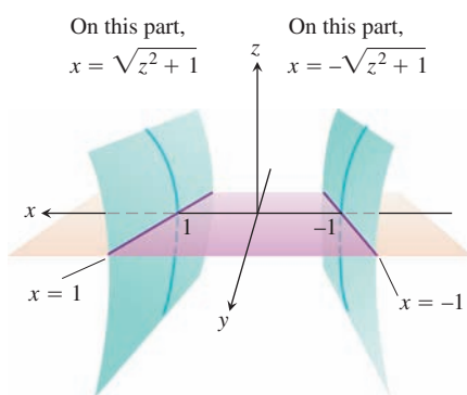
FIGURE 14.50 The region in the xy -plane from which the first two coordinates of the points (x, y, z) on the hyperbolic cylinder x^2 - z^2 = 1 are selected excludes the band -1 < x < 1 in the xy -plane (Example 2).
