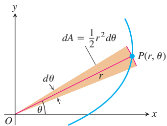
FIGURE 11.31 The area differential dA for the curve r = f(\theta) .
