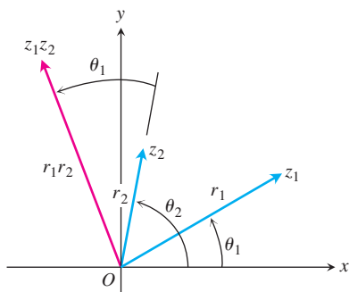
FIGURE A.26 When z_1 and z_2 are multiplied, |z_1 z_2| = r_1 \cdot r_2 and \arg(z_1 z_2) = \theta_1 + \theta_2 .
