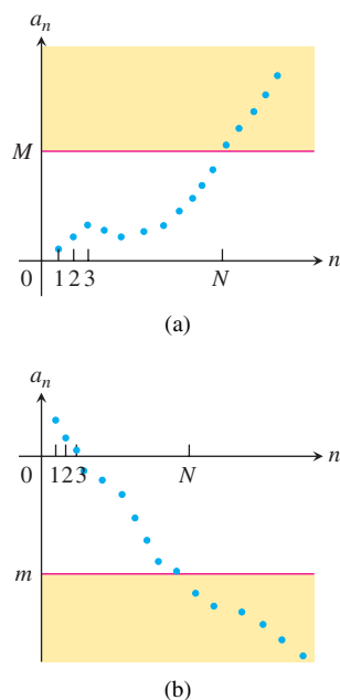
FIGURE 10.3 (a) The sequence diverges to \infty because no matter what number M is chosen, the terms of the sequence after some index N all lie in the yellow band above M . (b) The sequence diverges to -\infty because all terms after some index N lie below any chosen number m .
