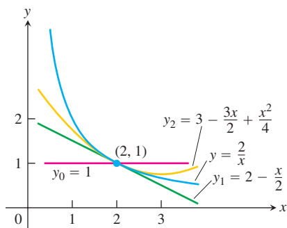
FIGURE 10.15 The graphs of f(x) = 2/x and its first three polynomial approximations (Example 2).
