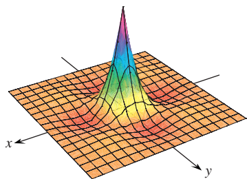
FIGURE 14.38 The function
