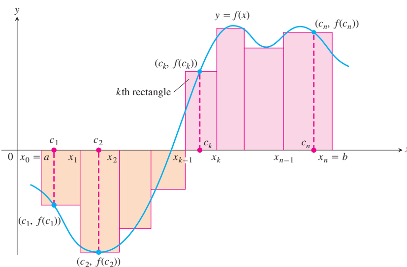
FIGURE 5.9 The rectangles approximate the region between the graph of the function y = f(x) and the x -axis. Figure 5.8 has been enlarged to enhance the partition of [a, b] and selection of points c_k that produce the rectangles.
