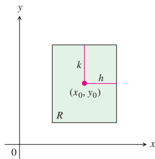
FIGURE 14.36 The rectangular region R : |x - x_0| \leq h , |y - y_0| \leq k in the xy -plane.
