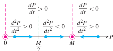
FIGURE 9.24 The completed phase line for logistic growth (Equation 6).
