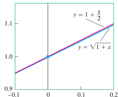
FIGURE 3.52 Magnified view of the window in Figure 3.51.
