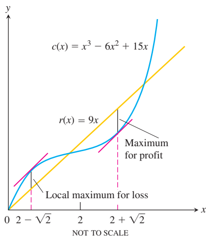
FIGURE 4.43 The cost and revenue curves for Example 5.
