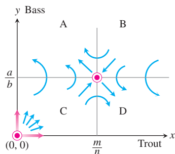
FIGURE 9.30 Motion along the trajectories near the rest points (0, 0) and (m/n, a/b) .
