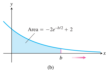
FIGURE 8.13 (a) The area in the first quadrant under the curve y = e^{-x/2} (b) The area is an improper integral of the first type.
