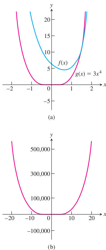
FIGURE 2.69 The graphs of f and g are (a) distinct for |x| small, and (b) nearly identical for |x| large (Example 19).
