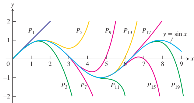
FIGURE 10.20 The polynomials
