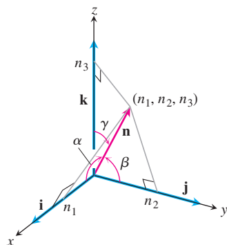
FIGURE 16.70 The components of \mathbf{n} are the cosines of the angles \alpha , \beta , and \gamma that it makes with \mathbf{i} , \mathbf{j} , and \mathbf{k} .
