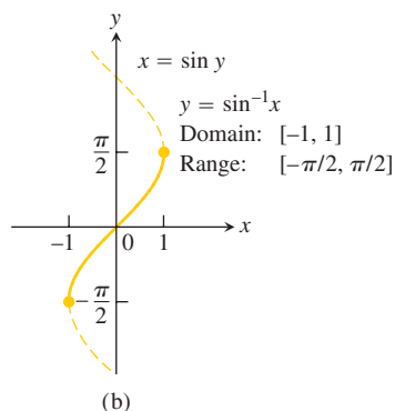
FIGURE 1.67 The graphs of (a) y = \sin x, -\pi/2 \leq x \leq \pi/2 , and (b) its inverse, y = \sin^{-1} x . The graph of \sin^{-1} x , obtained by reflection across the line y = x , is a portion of the curve x = \sin y .
