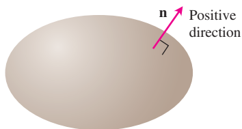
FIGURE 16.49 Smooth closed surfaces in space are orientable. The outward unit normal vector defines the positive direction at each point.
