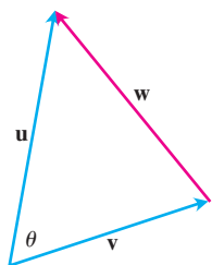
FIGURE 12.21 The parallelogram law of addition of vectors gives \mathbf{w} = \mathbf{u} - \mathbf{v} .
