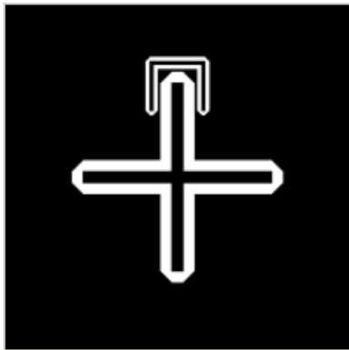
geometry (xmon + claw)
