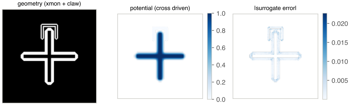
Figure 5: A sampled design, its solved potential (cross driven), and the surrogate's absolute error field.
