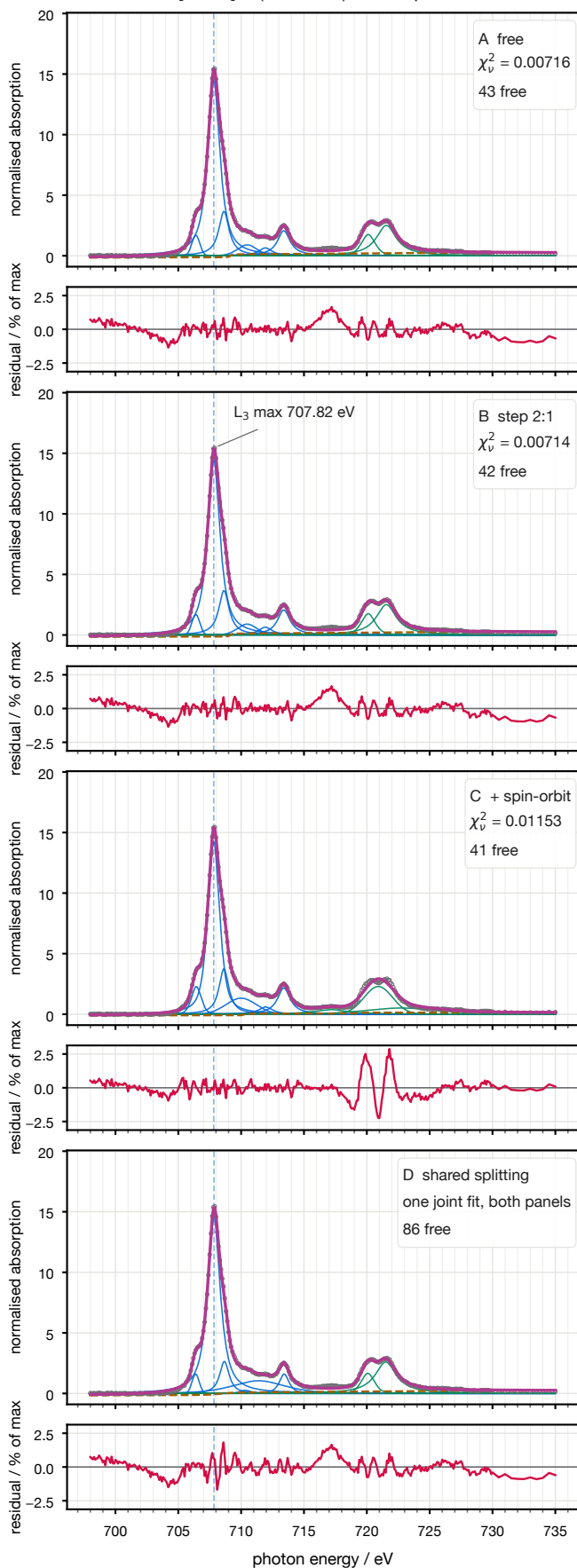
[\text{FeCl}_4]^- ( \text{Fe}^{3+} , d^5 ) — 331 points
