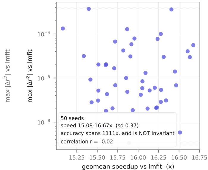
(B) across seeds, the two do not trade
