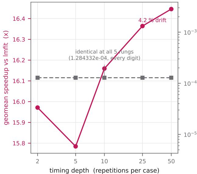
(A) depth moves speed, and cannot move accuracy
