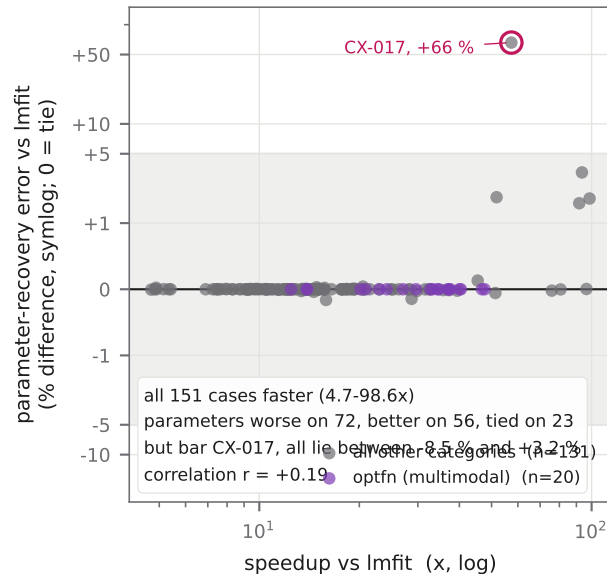
(C) per case, the trade never opens
