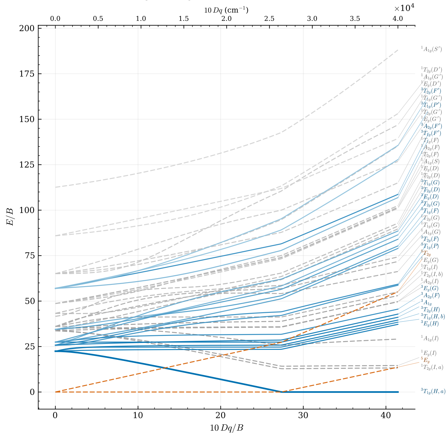
Tanabe-Sugano diagram, d^4 ( B = 965 , C = 4449 \text{ cm}^{-1} )
