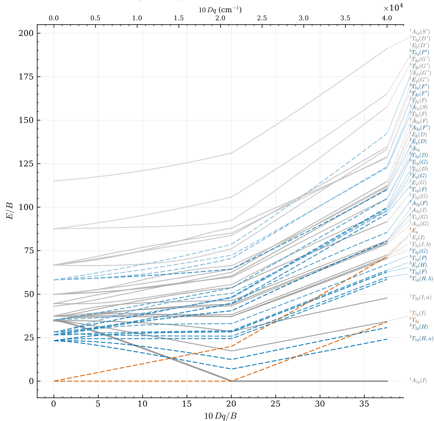
Tanabe-Sugano diagram, d^6(B = 1065, C = 5120 \text{ cm}^{-1})
