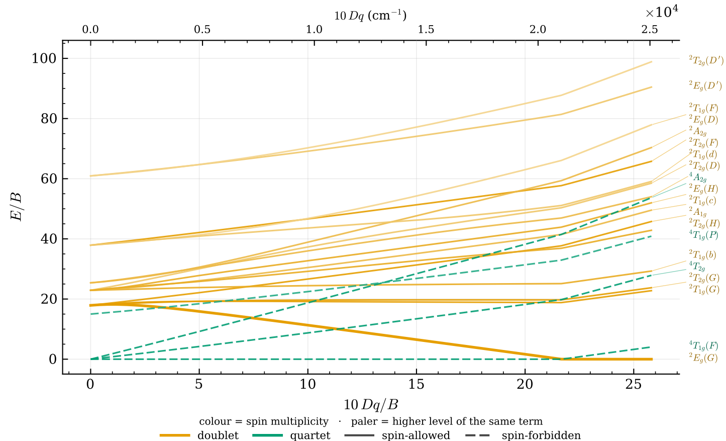
Tanabe-Sugano diagram, d^7 ( B = 971 , C = 4498 \text{ cm}^{-1} )
