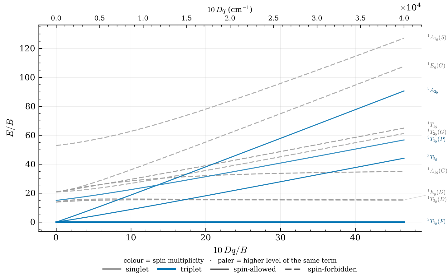
Tanabe-Sugano diagram, d^2 ( B = 860 , C = 3801 \text{ cm}^{-1} )
