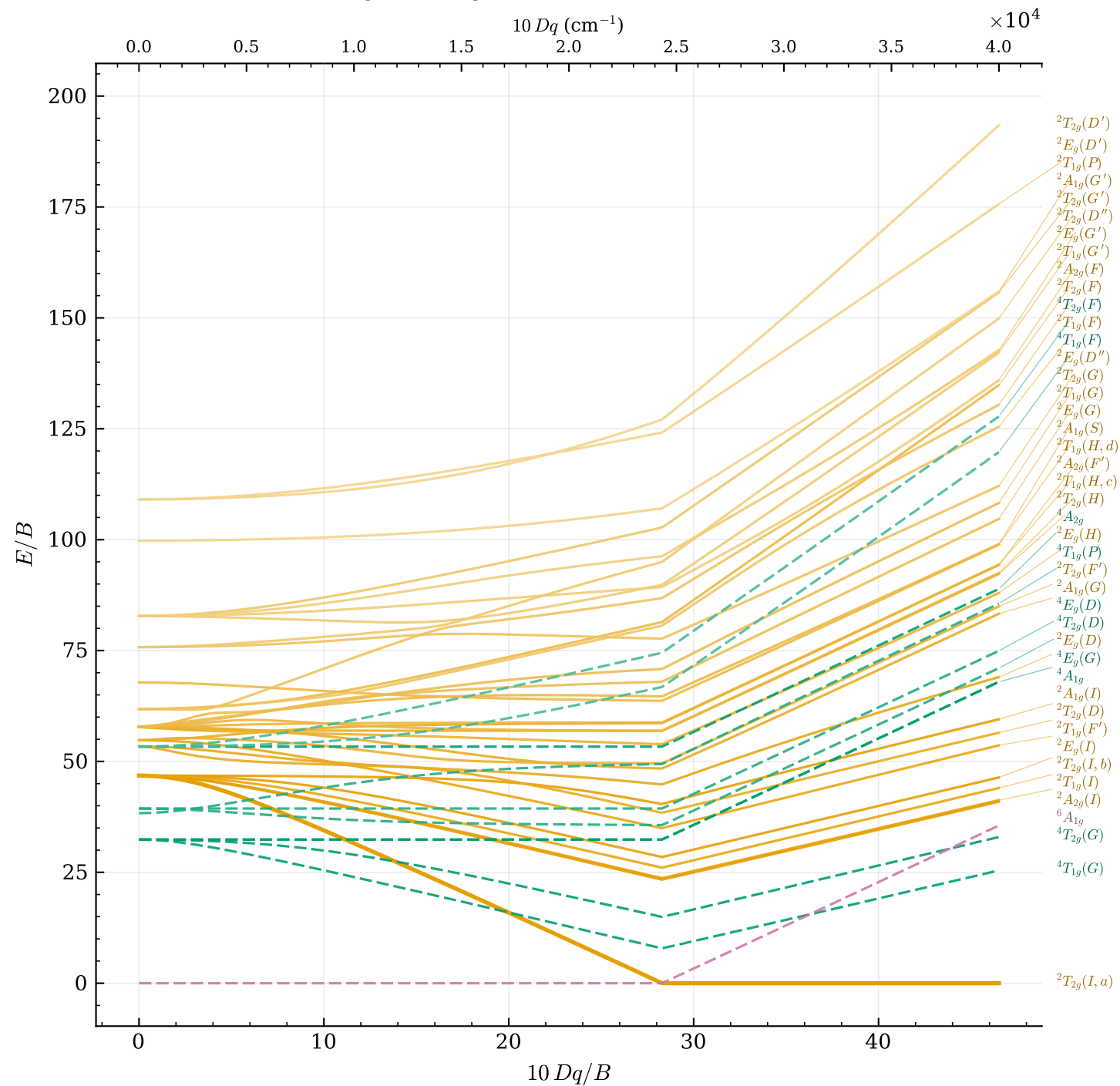
Tanabe-Sugano diagram, d^5 ( B = 860 , C = 3850 \text{ cm}^{-1} )
