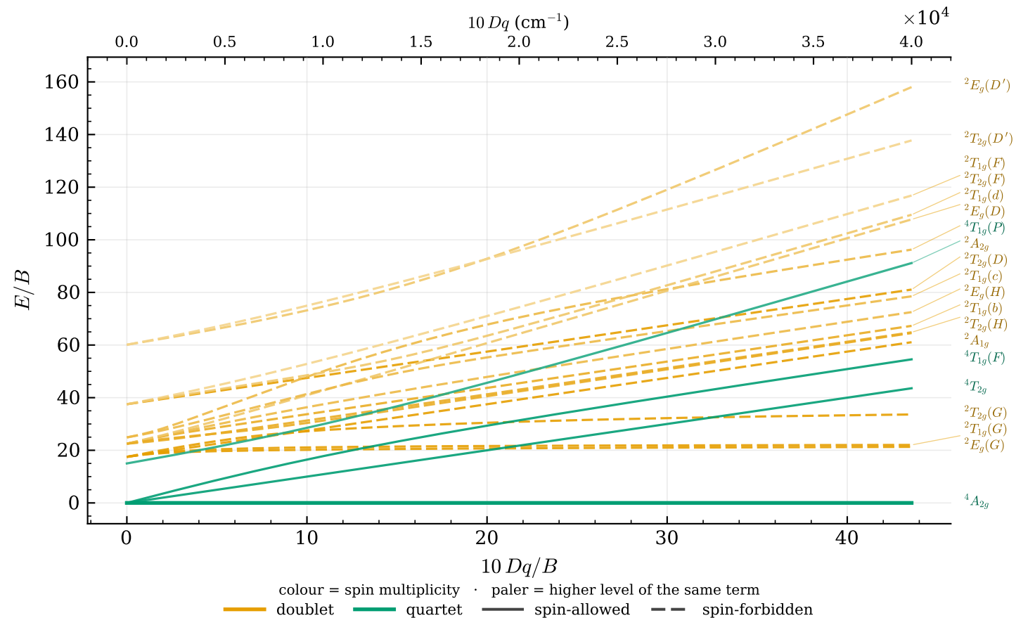
Tanabe-Sugano diagram, d^3 ( B = 918, C = 4132 \text{ cm}^{-1} )
