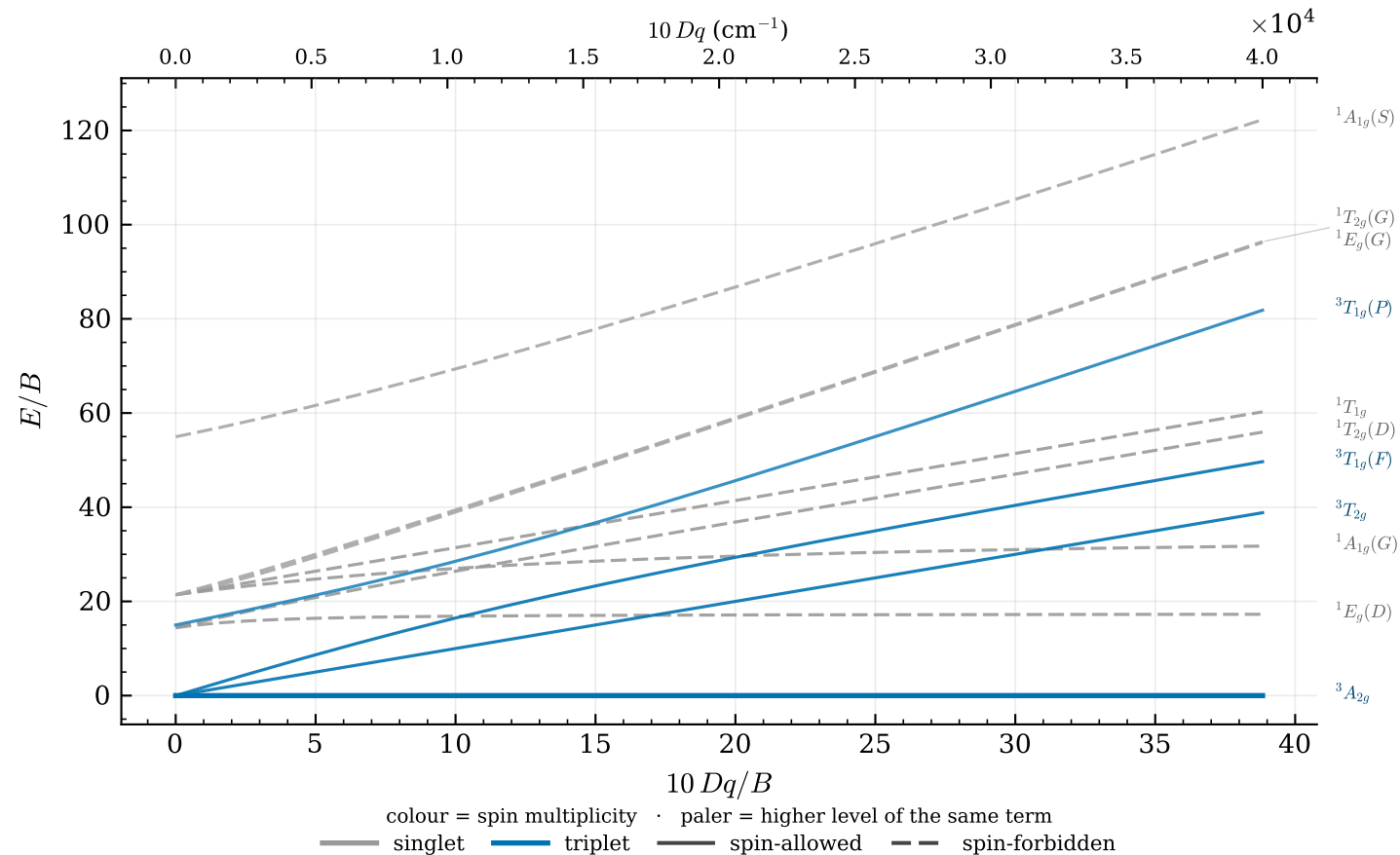
Tanabe-Sugano diagram, d^8 ( B = 1030 , C = 4850 \text{ cm}^{-1} )
