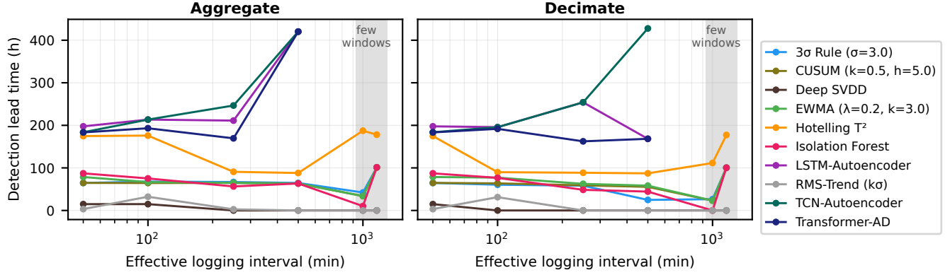
Figure 3. Detection lead time vs effective SCADA logging interval on IMS (controlled sweep, mean across runs): aggregation (left) and decimation (right). Shading marks the few-windows regime at the two largest factors, where only one or two runs remain.
