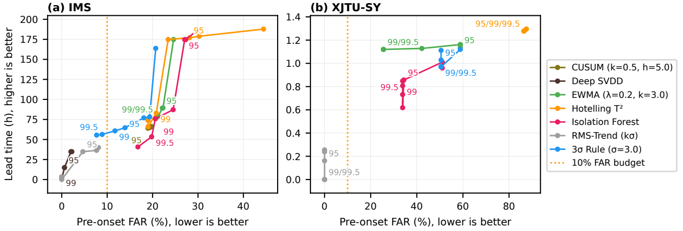
Figure 5. Lead-time vs pre-onset-FAR trade-off, threshold percentile swept (mean across runs): (a) IMS, (b) the ten XJTU-SY bearings; labels mark the 95th, 99th and 99.5th-percentile operating points (tabulated for IMS in Table 9) where they fit legibly. Up and to the left is better.
