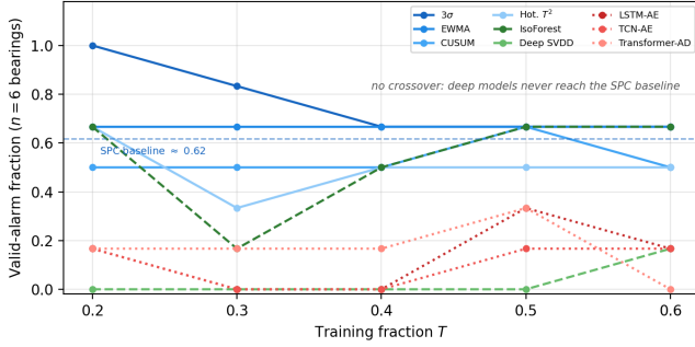
Figure 6. Valid-alarm fraction vs. training fraction T on FEMTO ( n = 6 ): SPC charts in blue, deep reconstruction models in red, Deep SVDD separately; dashed: the SPC baseline ( \approx 0.62 ). The three N/A cells at T = 0.20 (Bearing3_1, 20 training windows) count as no valid alarm.
