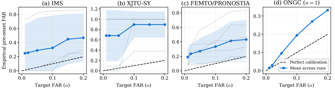
Figure 4. Conformal calibration: empirical pre-onset FAR vs target \alpha for (a) IMS, (b) XJTU-SY, (c) FEMTO/PRONOSTIA and (d) the ONGC turbine ( n = 1 case study, Appendix D.2). Points on or below the diagonal satisfy the distribution-free guarantee; bearings with only one or two pre-onset windows are flagged uncalibrated. Panel (a) empirical FAR at \alpha = 0.01, 0.05, 0.10, 0.20 : test 1 0.74, 0.82, 0.85, 0.86; test 2 0.00, 0.00, 0.00, 0.25; test 3 0.01, 0.04, 0.13, 0.30.
