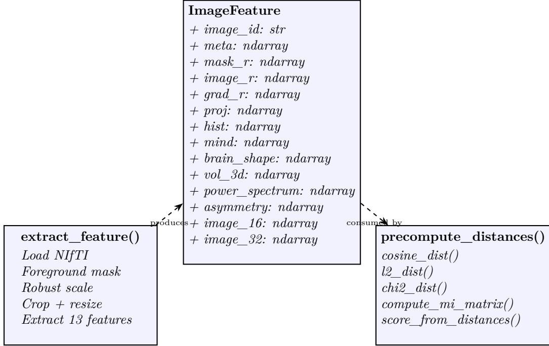
Figure 4: UML class diagram of the feature extraction system.
