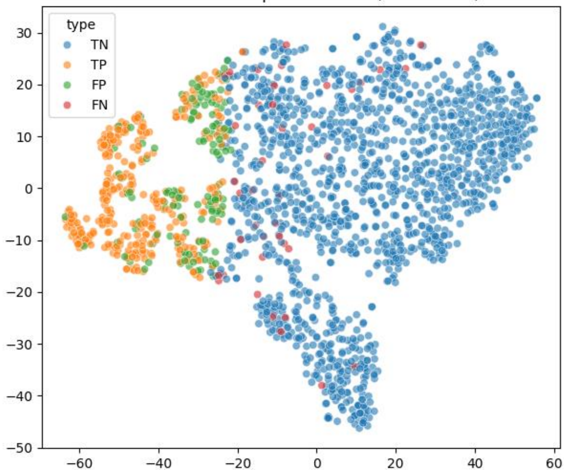
t-SNE of Fused Representations (Error-Aware)
