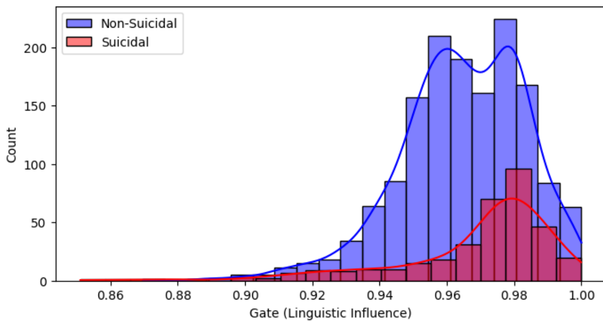
Gate Value Distribution
