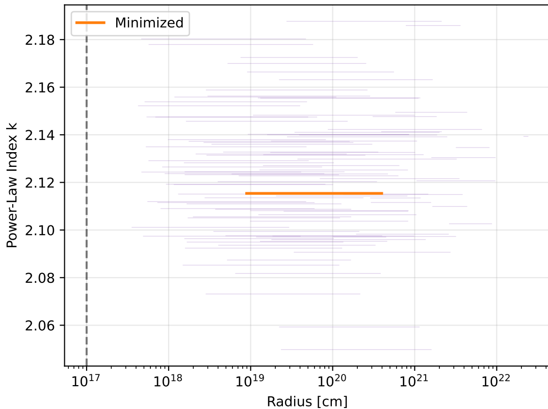
Power-Law Index Profile
