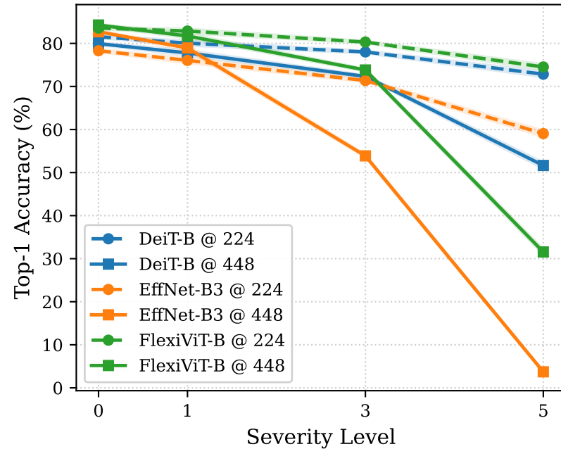
Gaussian Noise
