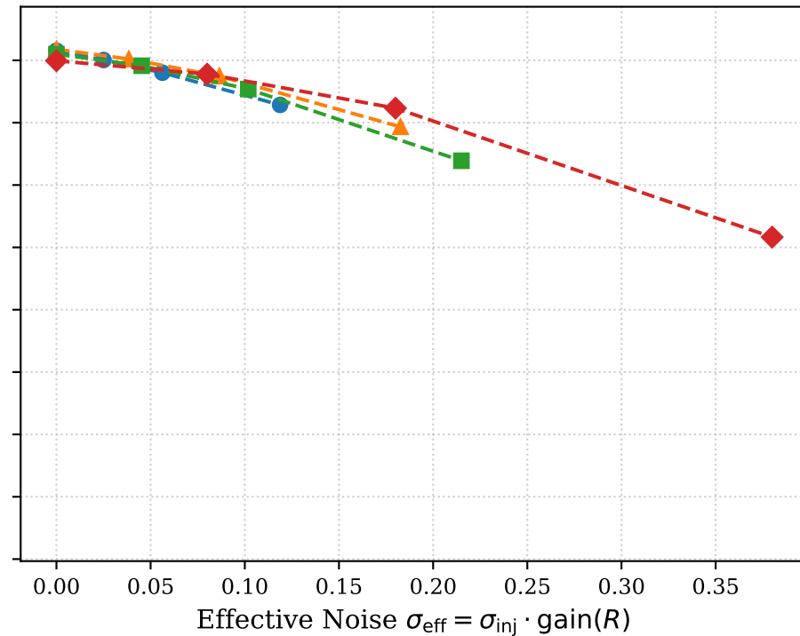
DeiT-B/16
