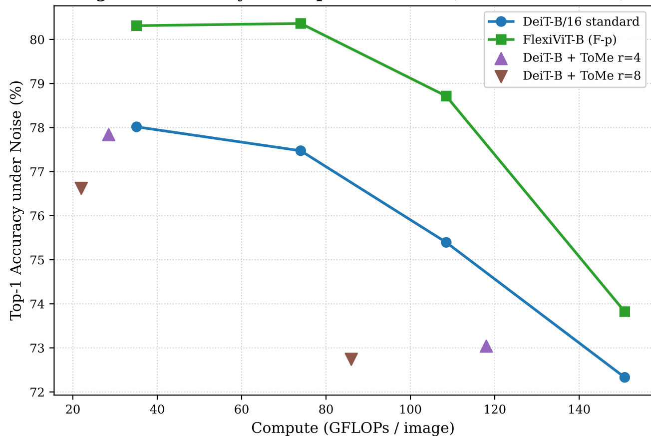
Figure 3: Accuracy vs Compute Trade-off (Gaussian Noise s3)
