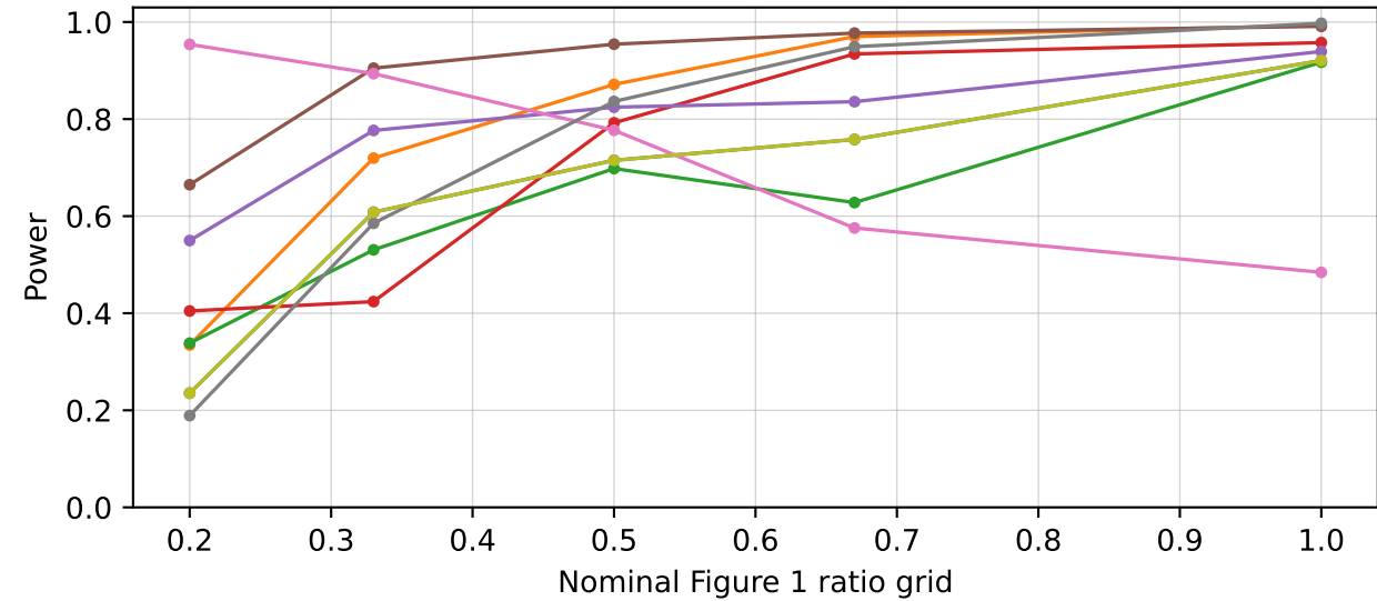
Asian put, 12 observations: GradTwo median estimated power
