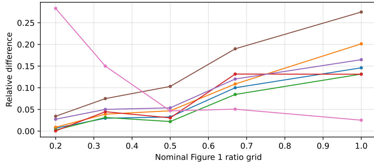
Asian call, 4 observations: relative median price difference
