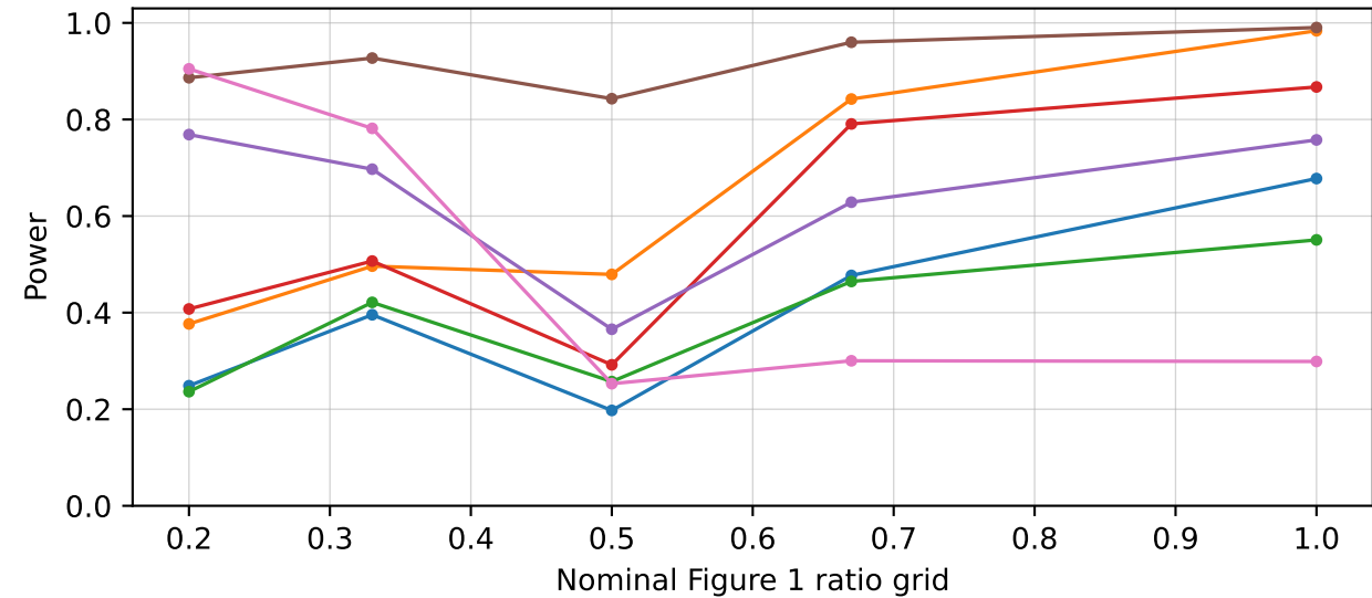
Asian call, 4 observations: GradTwo median estimated power
