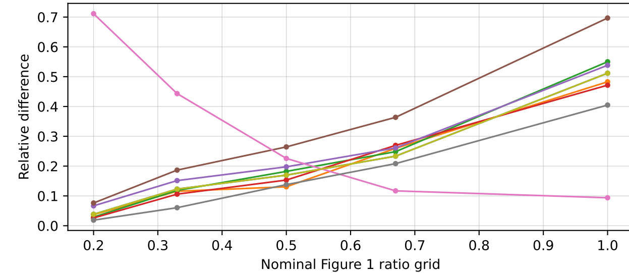
Asian put, 12 observations: relative median price difference
