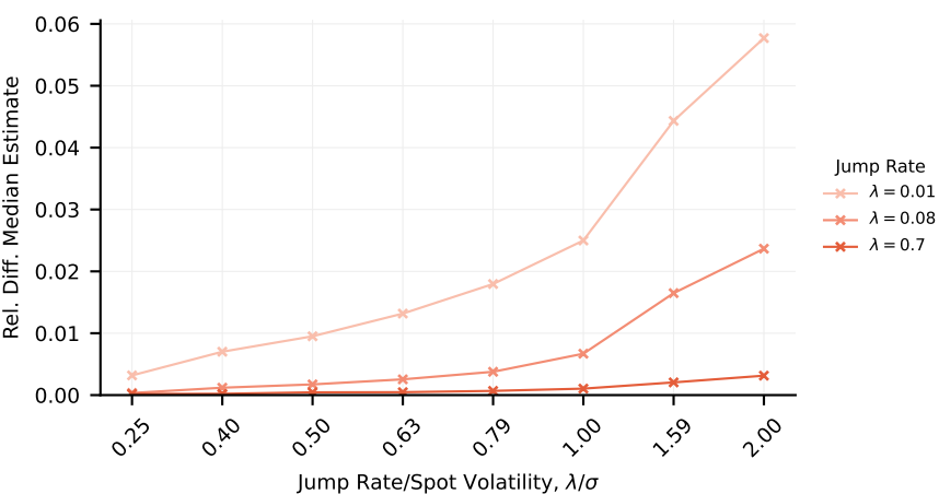
(a) GBM Model vs. Merton Model, Vanilla Call Option
