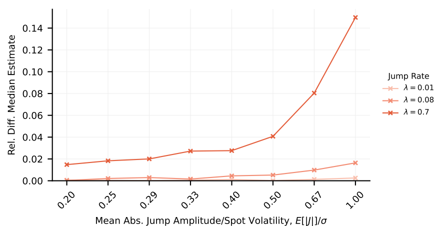
(b) Vasicek Model vs. MRJD Model, Vanilla Put Option
