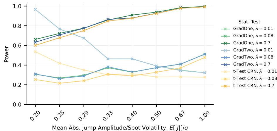
Hypothesis Tests: Median Power Estimate to Option Value Difference. Asian Call Option, 4 observations. 256 Paths/Estimate. Vasicek Model vs. MRJD Model. Two-sided Test.
