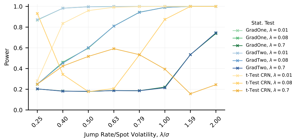
Hypothesis Tests: Median Power Estimate to Option Value Difference. Vanilla Call Option. 16384 Paths/Estimate. GBM Model vs. Merton Model. Two-sided Test.
