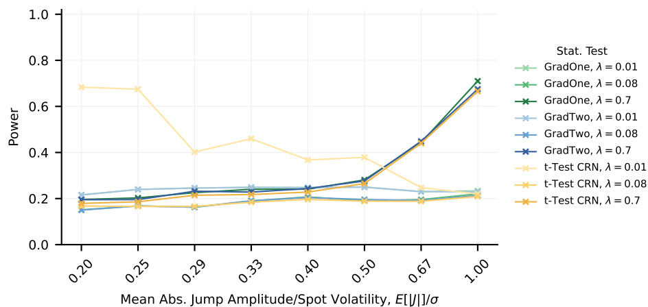
Hypothesis Tests: Median Power Estimate to Option Value Difference. Vanilla Put Option. 256 Paths/Estimate. Vasicek Model vs. MRJD Model. Two-sided Test.
