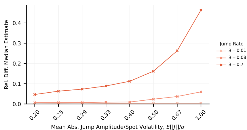
(c) Vasicek Model vs. MRJD Model, Asian Call Option, 4 observations
