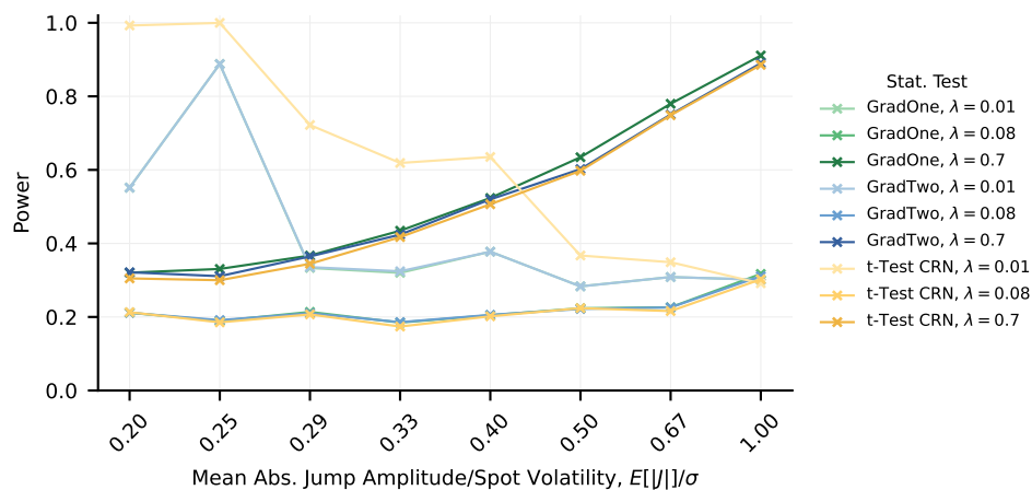
Hypothesis Tests: Median Power Estimate to Option Value Difference. Asian Put Option, 12 observations. 256 Paths/Estimate. Vasicek Model vs. MRJD Model. Two-sided Test.
