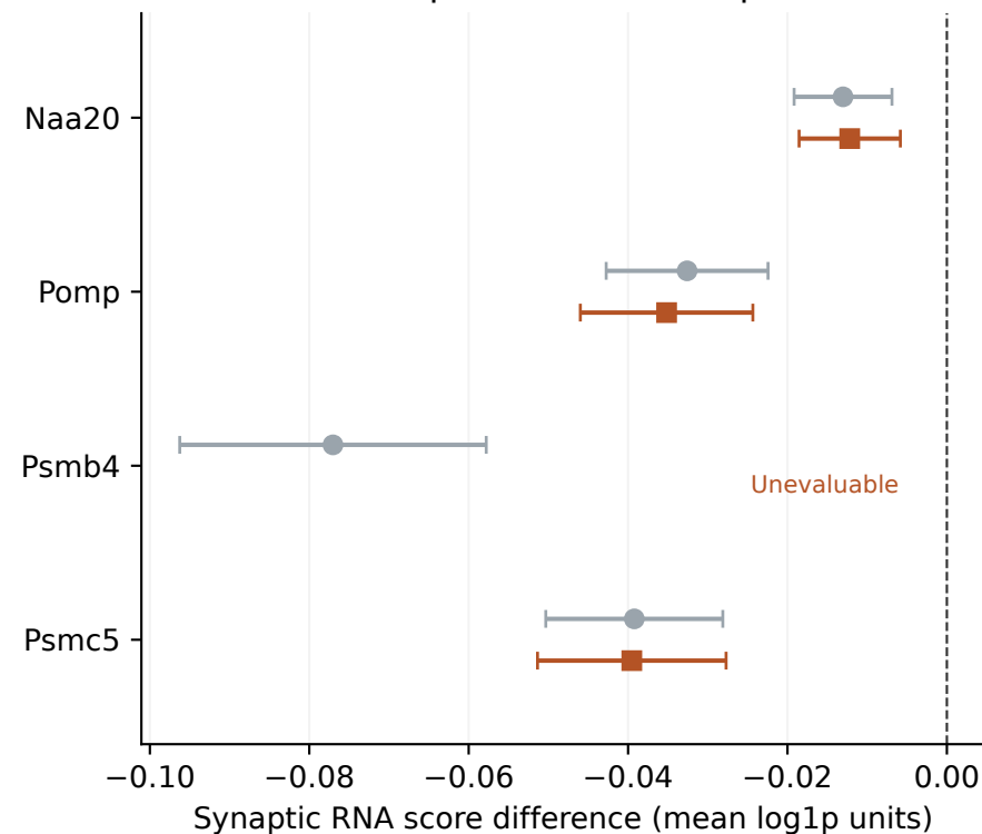
B Mouse perturbation comparison
