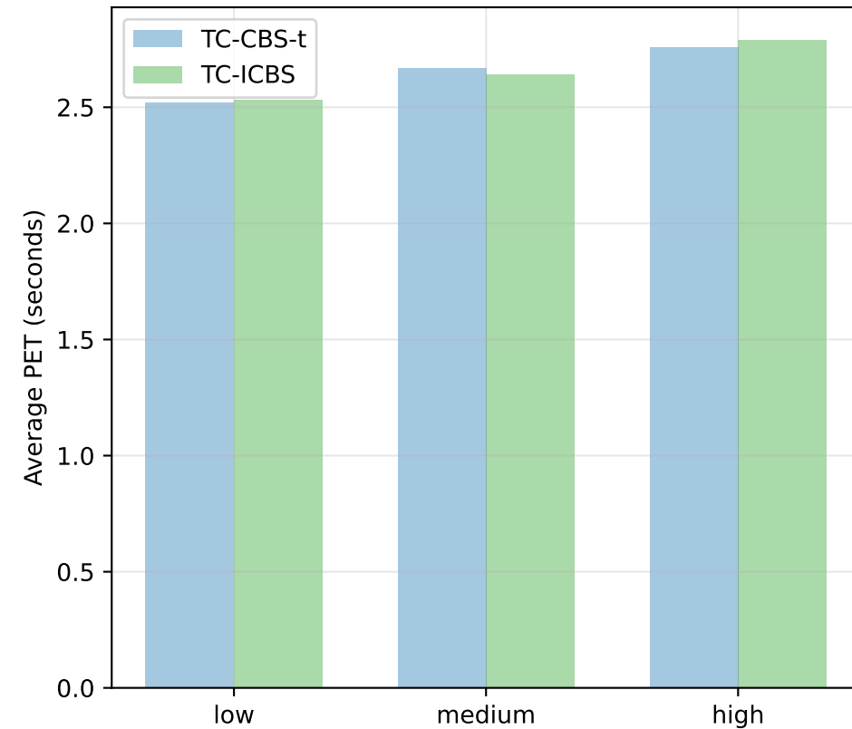
Post-Encroachment Time (PET)
