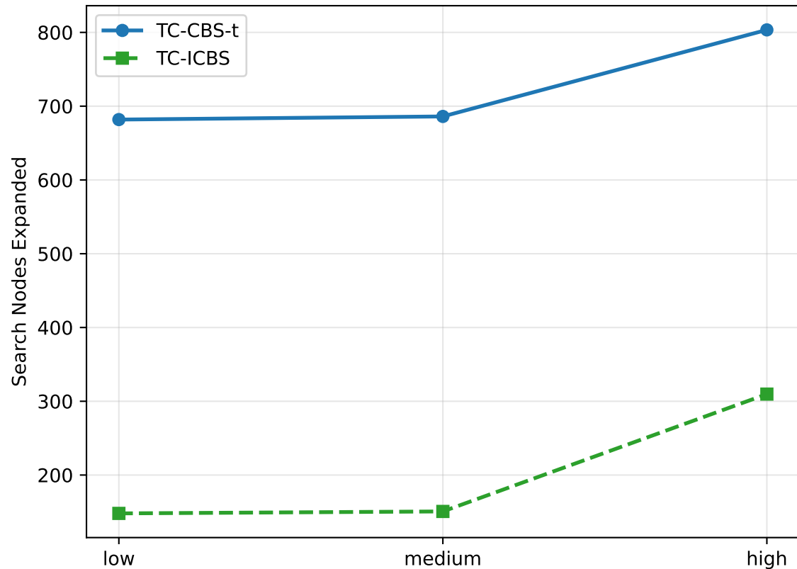
Search Nodes Expanded vs. Pedestrian Density
