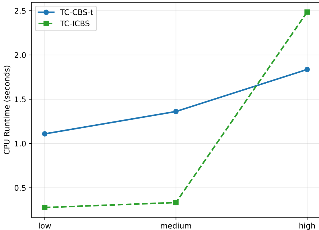
CPU Runtime vs. Pedestrian Density
