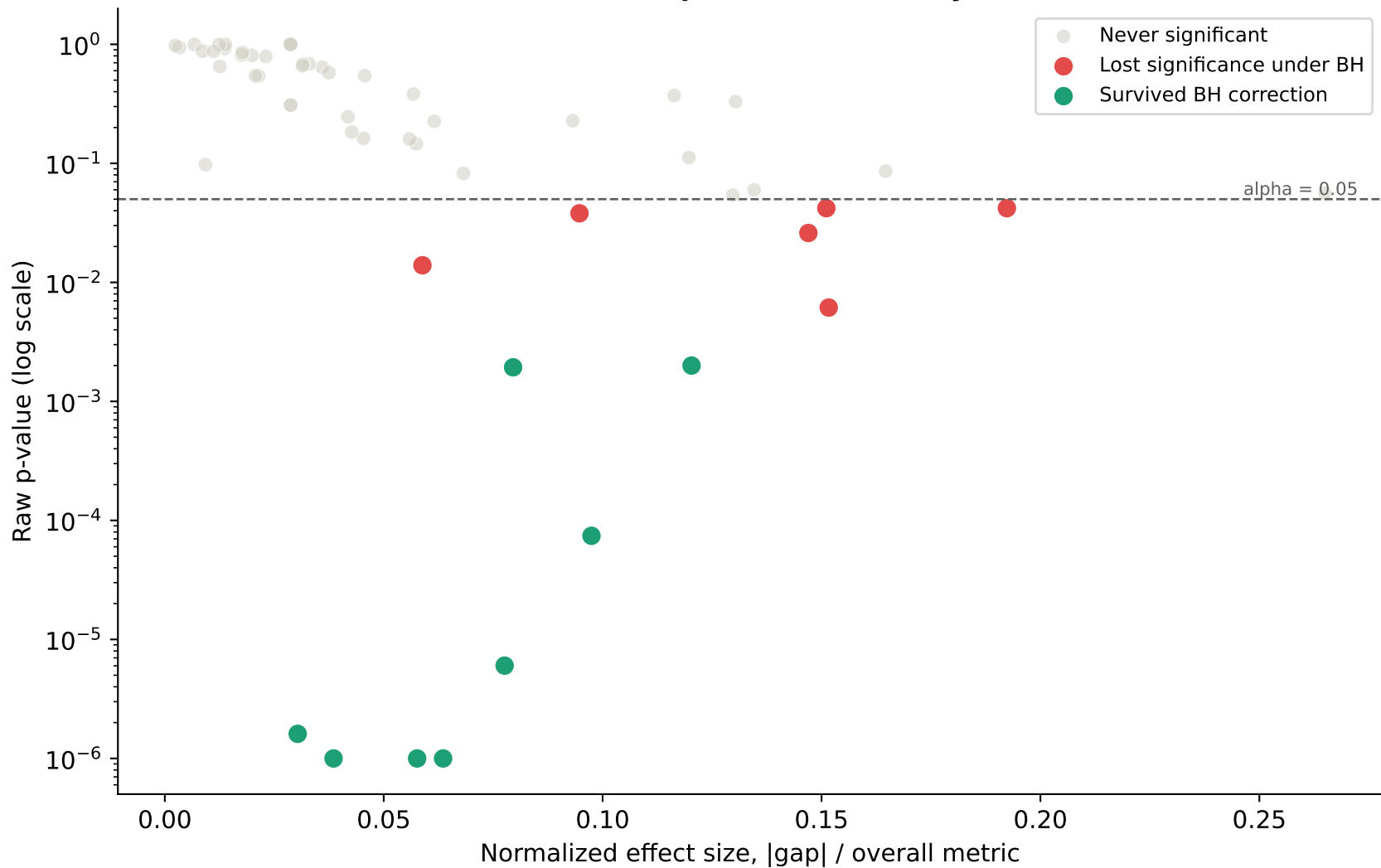
Normalized effect size vs raw p-value, colored by correction outcome
