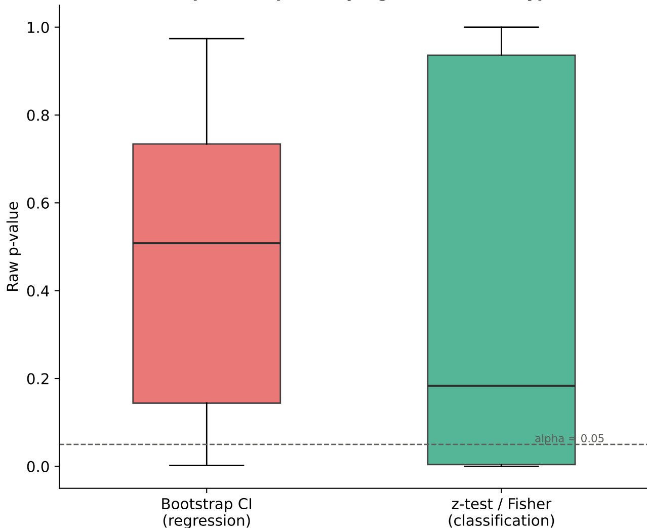
Raw p-value spread by significance test type
