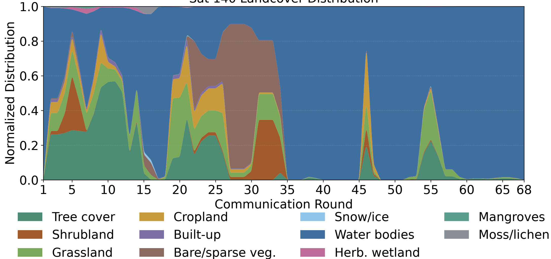
Sat 140 Landcover Distribution
