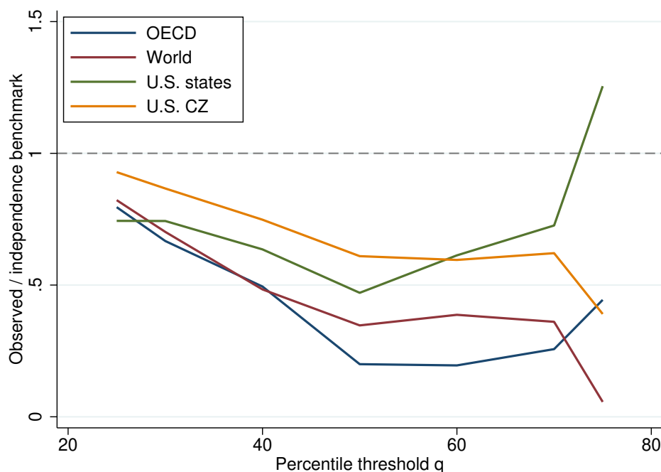
Figure A.7. Robustness to Percentile Thresholds
