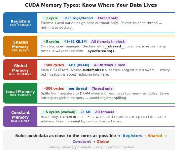
Figure 4: CUDA Memory Types
