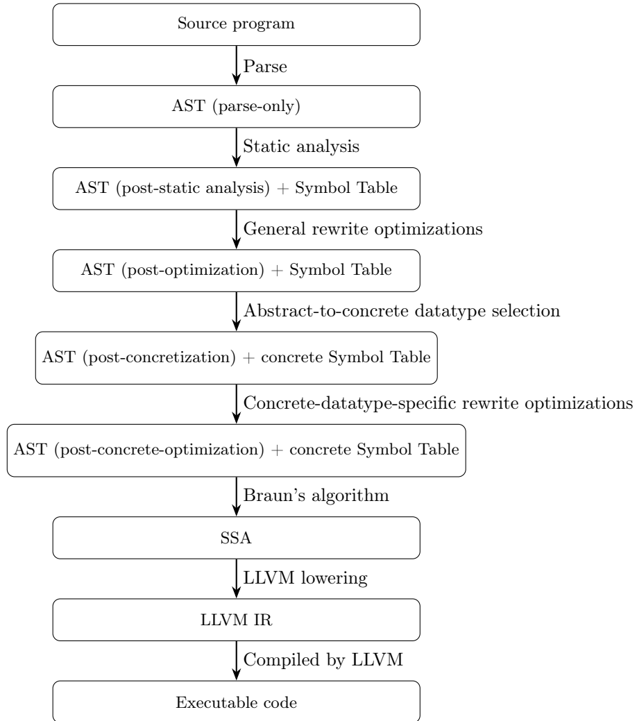
Figure 1: Simile compilation pipeline from source code to LLVM-based executable
