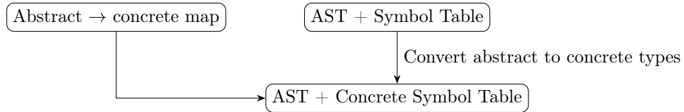
Figure 6: Component Diagram: Abstract Data Type Concretization (Scrappy version)
