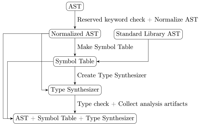
Figure 3: Component Diagram: Static Analysis
