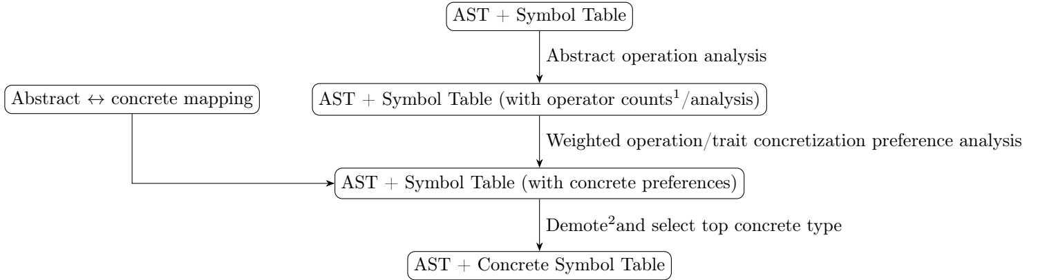
Figure 5: Component Diagram: Abstract Data Type Concretization
