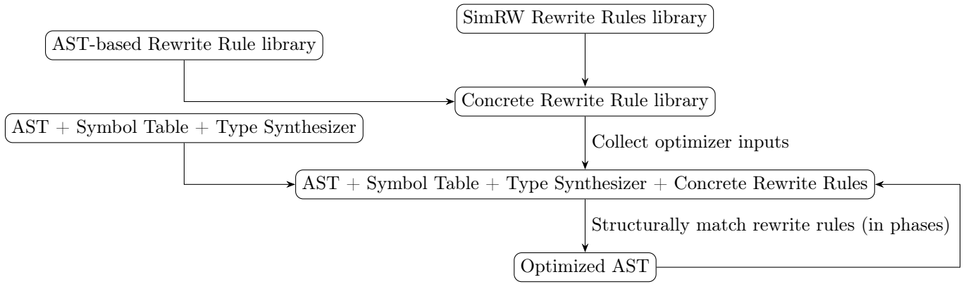
Figure 7: Component Diagram: Concrete-specific Rewrite Optimizations
