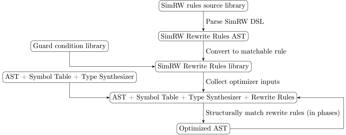
Figure 4: Component Diagram: General Rewrite Optimization
