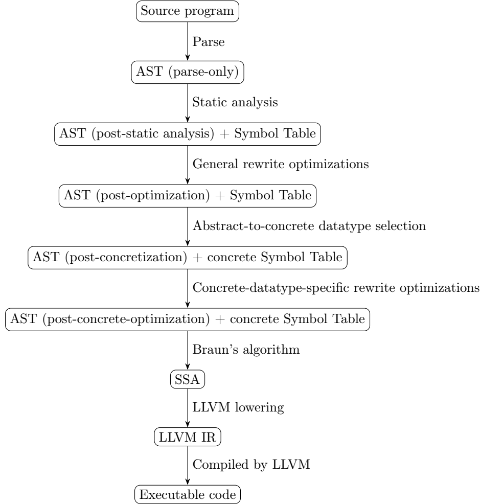
Figure 1: Simile compilation pipeline from source code to LLVM-based executable
